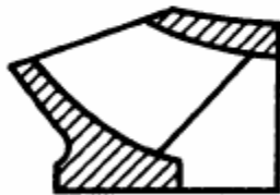
Fig. 5 Single or multistage single suction centrifugal pumps, in volute or diffuser-type casings with mixed flow impellers, deliver high capacity at low head. Specific speed range is 4000 to 6000.
