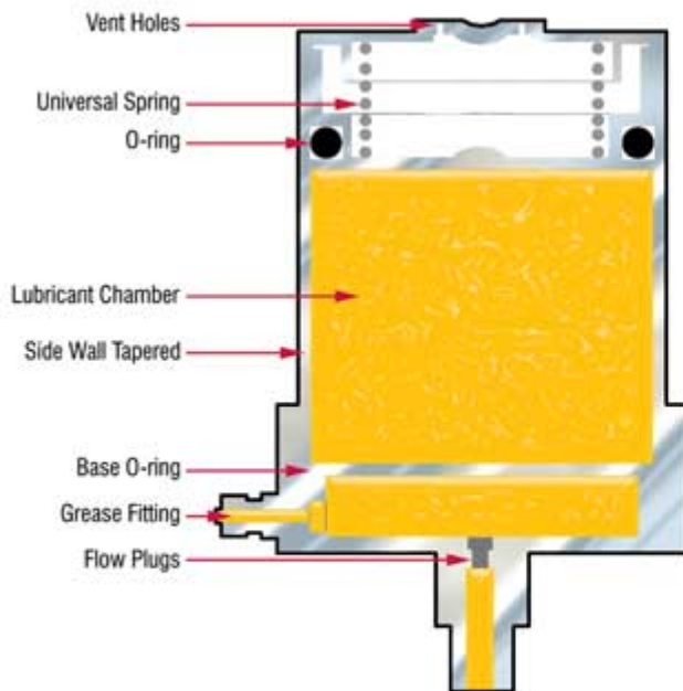
Figure 1. Original Single-Point Lubricator 2
