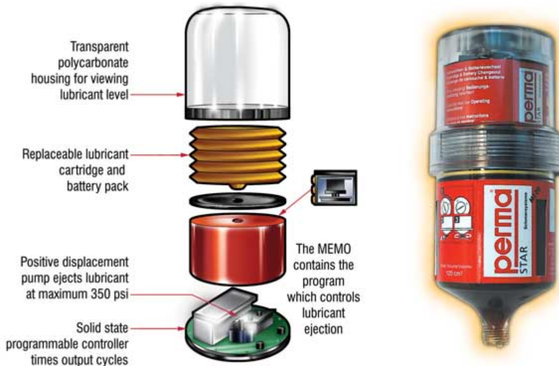
Figure 3. Electromechanical Unit 6
