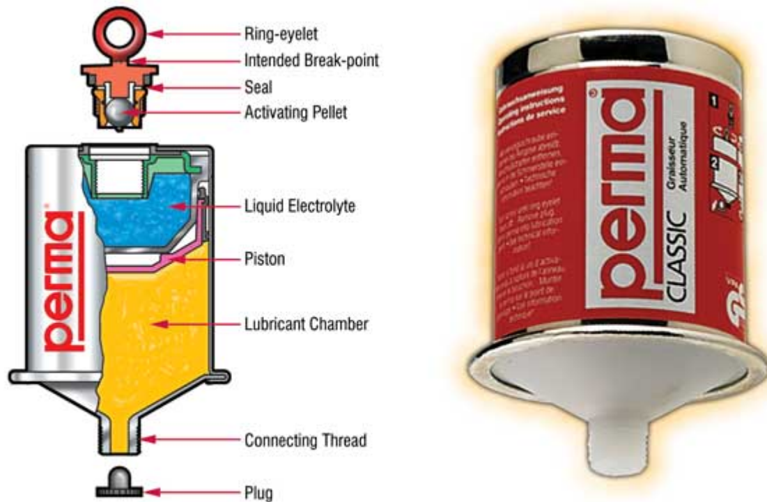
Figure 2. Single-Point Piston-Activated Lubricator 6
